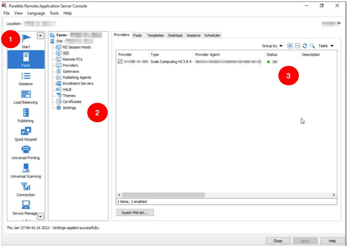
Parallels RAS Console general overview
